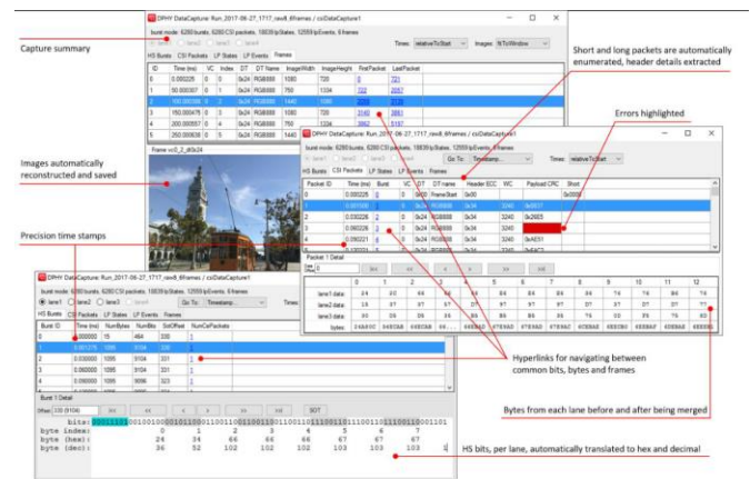
SV3C-DPRX screen capture illustrating CSI-2 over D-PHY protocol analysis of received packet data
