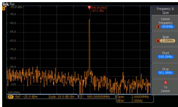
Figure 16: Strong 900 MHz radiation detected at the FPGA.
