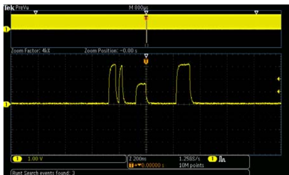
Figure 4: Runt pulses captured with runt triggering
