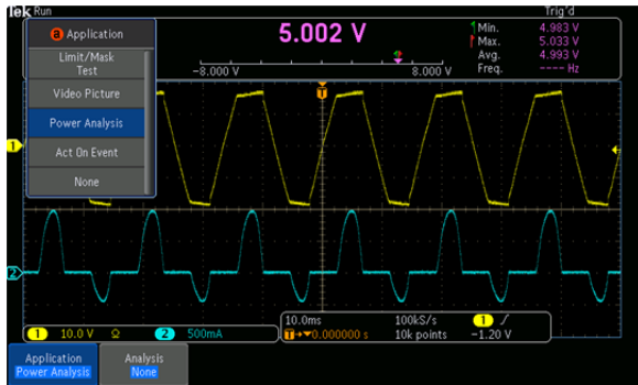
Figure 27: Selecting automated power measurements.
