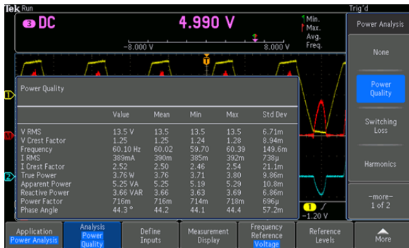
Figure 28: Power Supply input power quality measurements.
