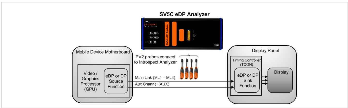
Figure 15: Typical application of the SV5C-eDP Analyzer and PV2 Probes connected to an Embedded DisplayPort. System.
